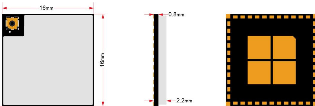
Figure 3: CQM74x-0-50-0U Module View
