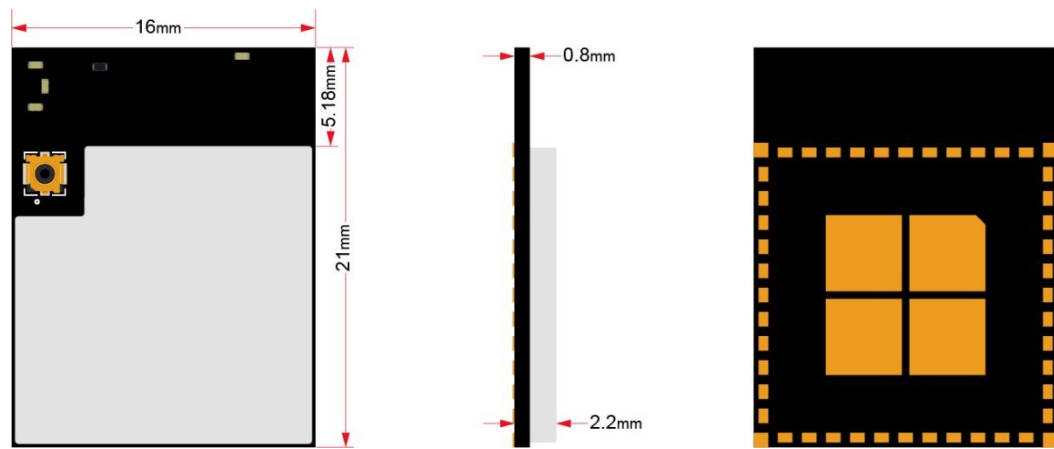
Figure 2: CQM74x-0-50-0B Module View
