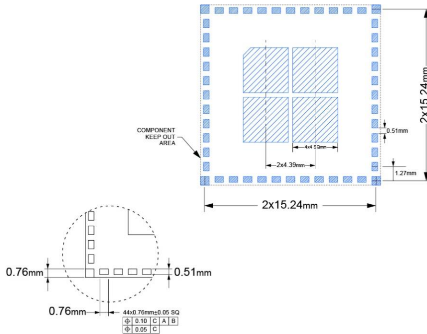
Figure 14: CQM74x-0-50-0U Module PCB Landing Pattern
