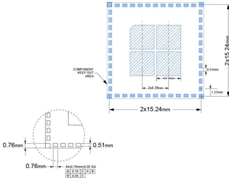
Figure 10: CQM74x-0-50-0P Module PCB Landing Pattern
