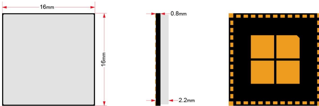
Figure 1: CQM74x-0-50-0P Module View
