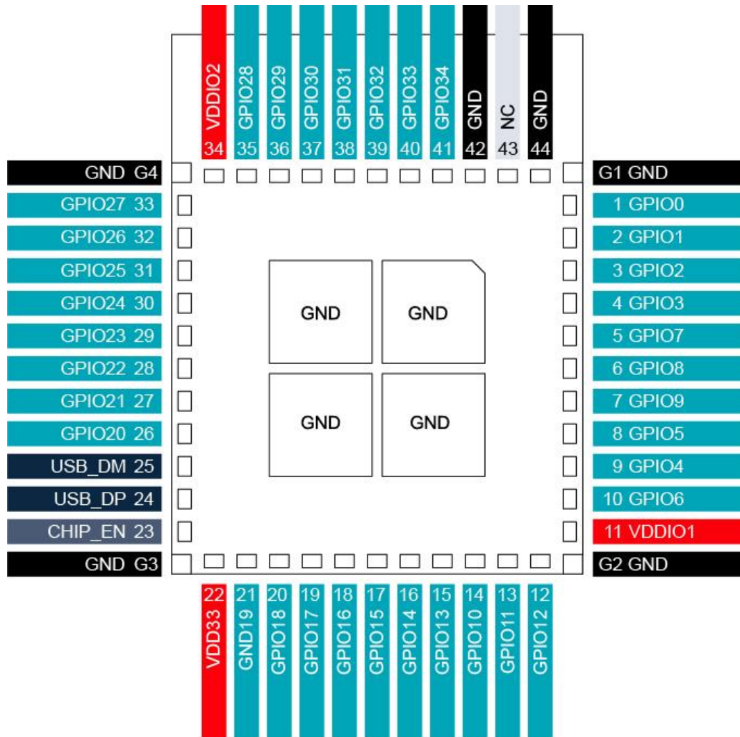
Figure 7: CQM74x-0-50-0B/U Module Pin Map
