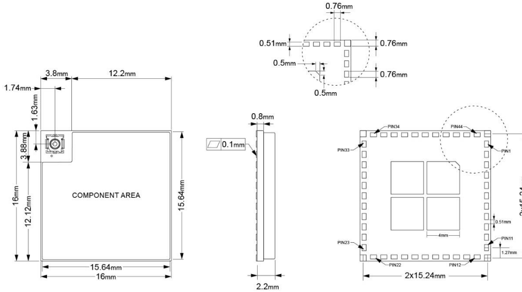
Figure 13: CQM74x-0-50-0U Module Dimension
