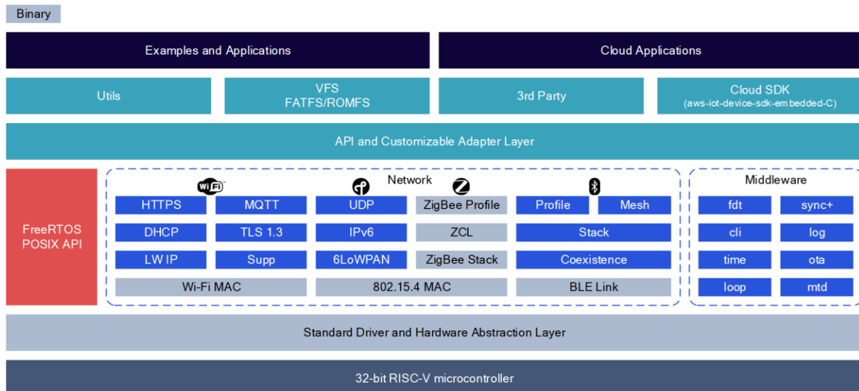
Figure 8: Computing Subsystem Software Architecture
