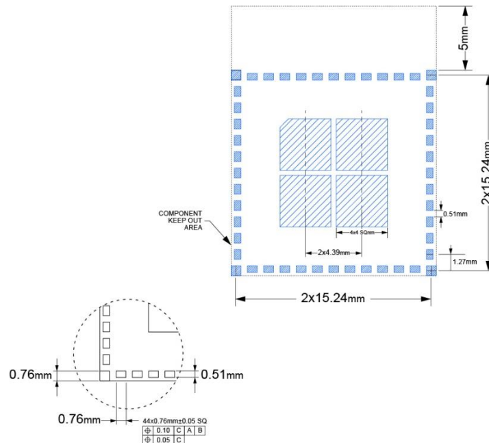
Figure 12: CQM74x-0-50-0B Module PCB Landing Pattern
