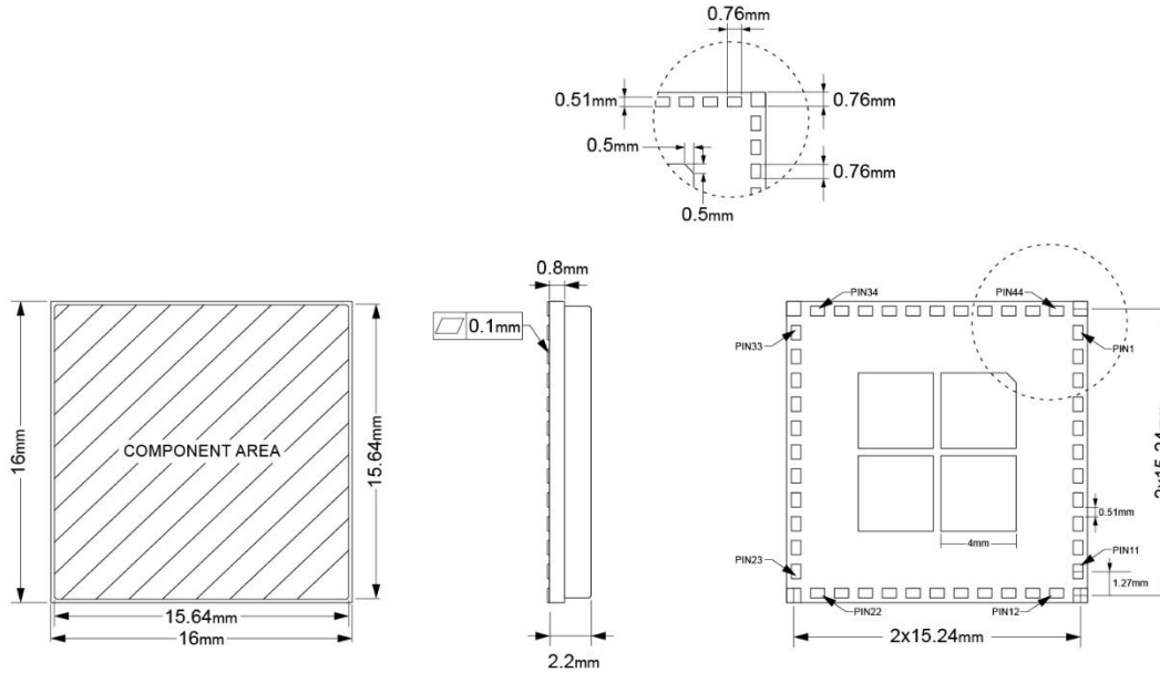
Figure 9: CQM74x-0-50-0P Module Dimension
