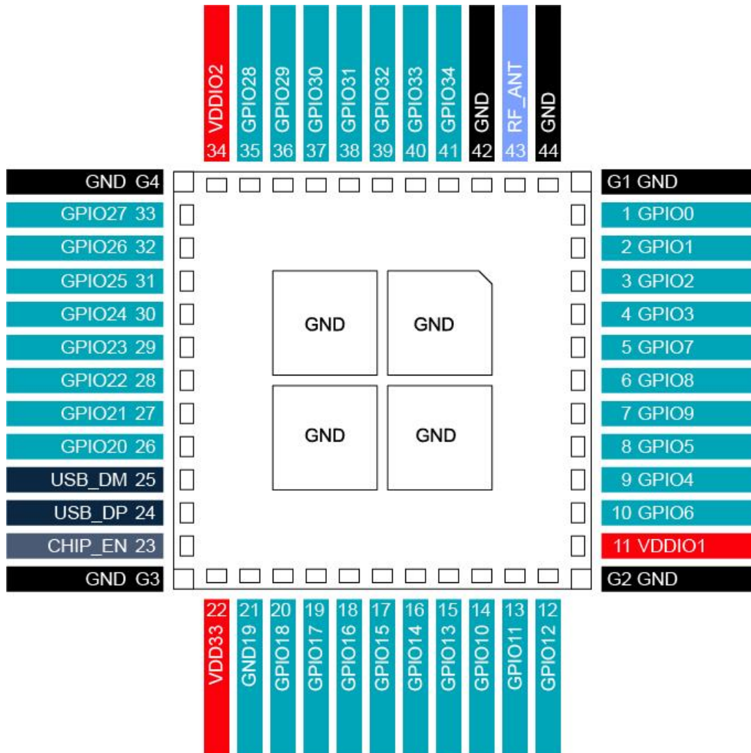
Figure 6: CQM74x-0-50-0P Module Pin Map
