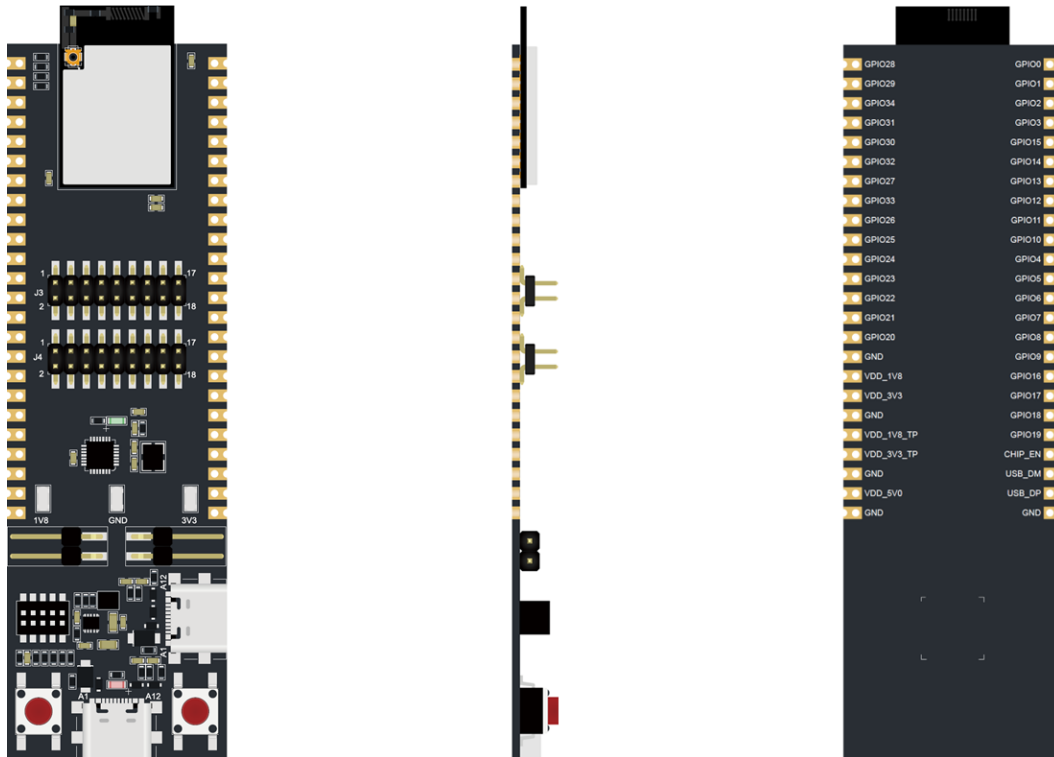
Figure 4: CQM74x Module Development Kit
