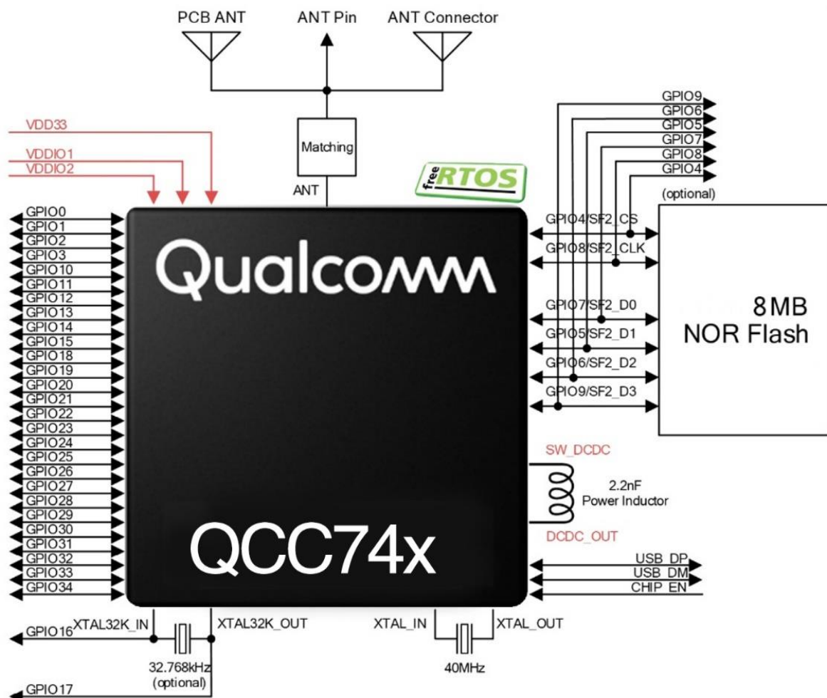
Figure 5: CQM74x Module Block Diagram
